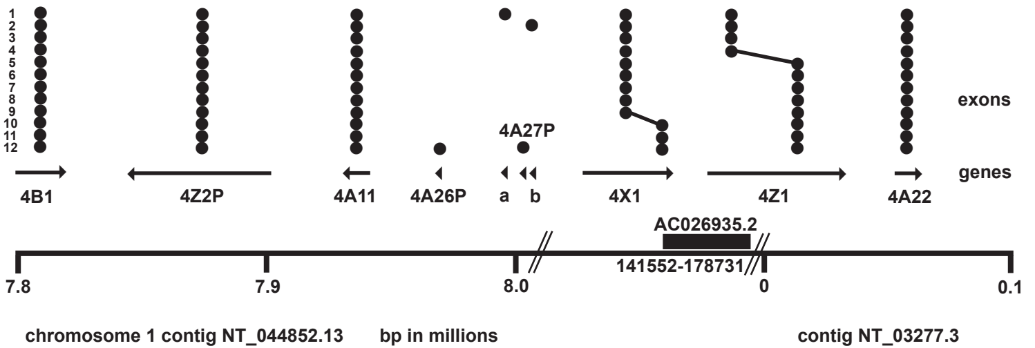
CYP4ABXZ locus in human April 2, 2003 D. Nelson (based on NCBI build 30)
