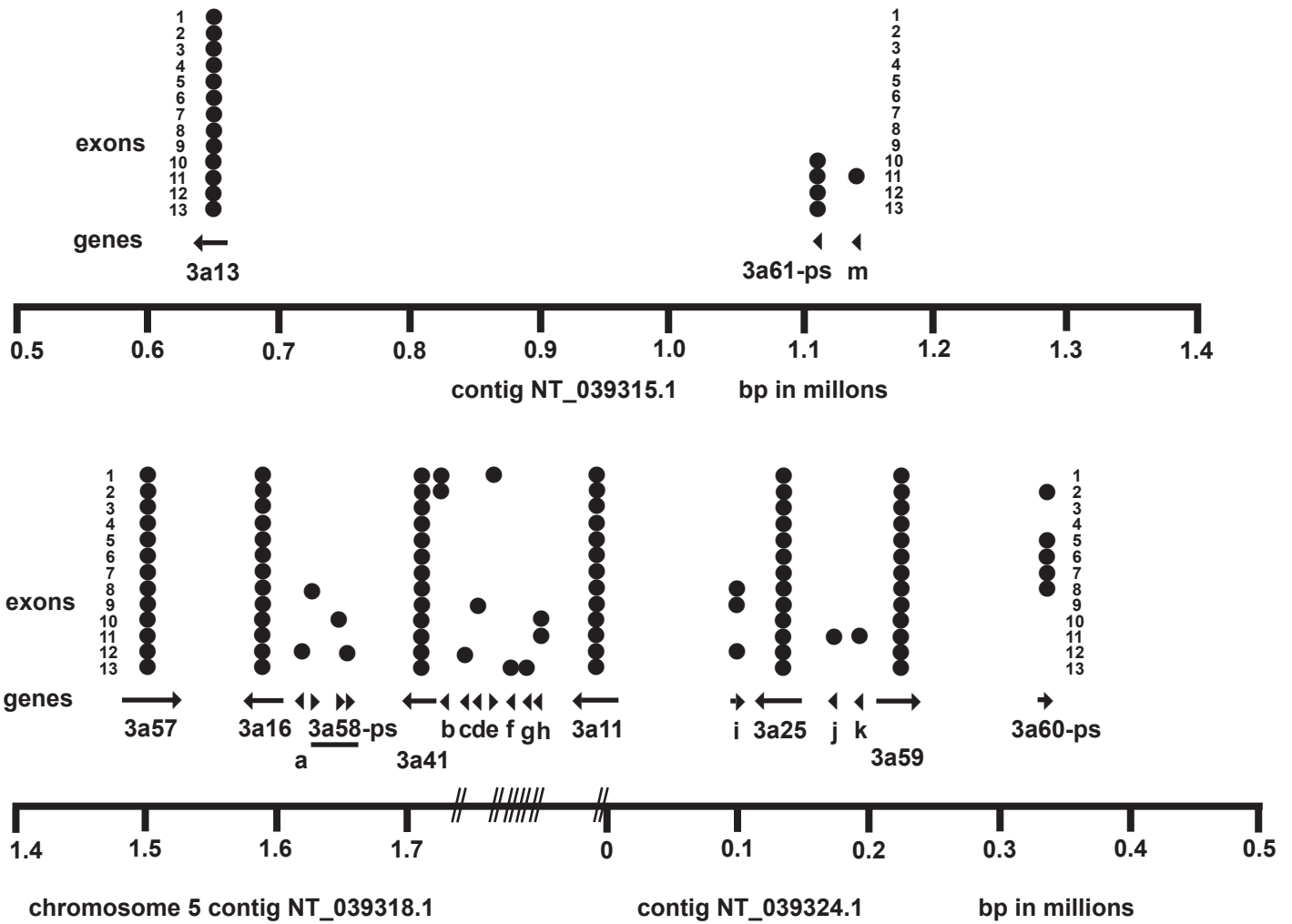
Cyp3a locus in mouse March 25, 2003 D. Nelson (based on NCBI build 30)
