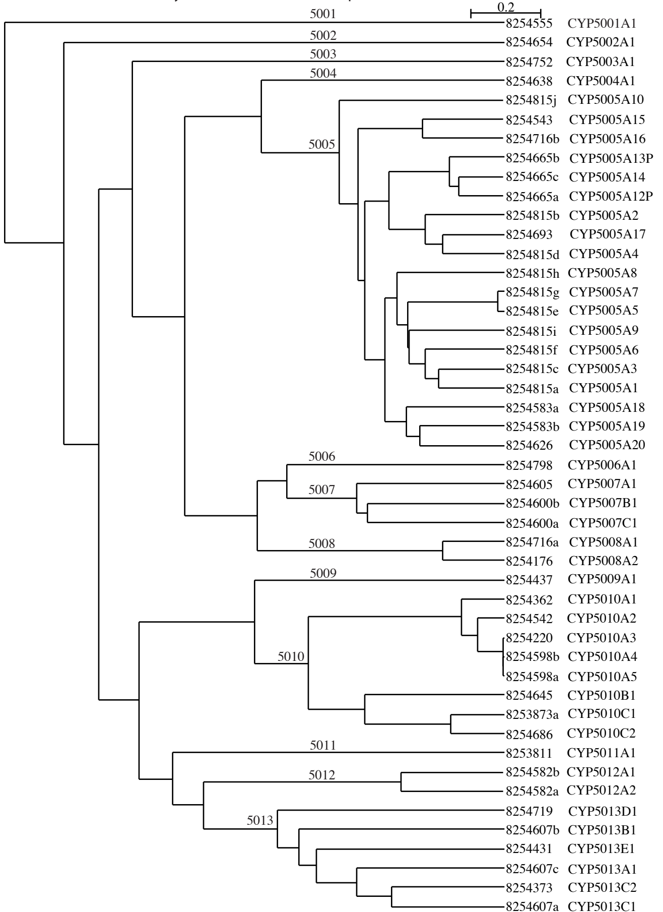
Revised UPGMA tree of 47 Tetrahymena P450s. D.Nelson April 22, 2004 Numbers are TIGR accessions
